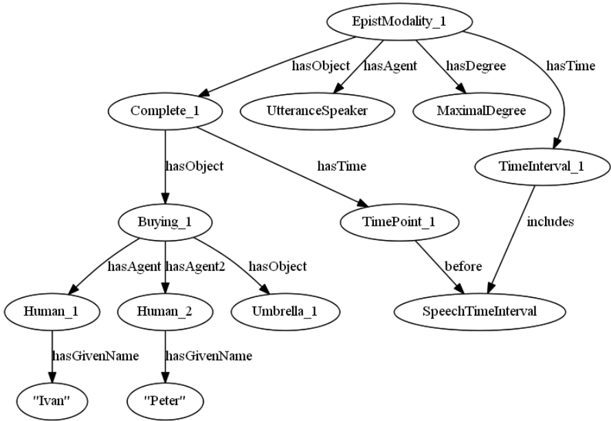
Fig. 1. Basic semantic graph for a sentence 'Ivan bought an umbrella from Peter'
